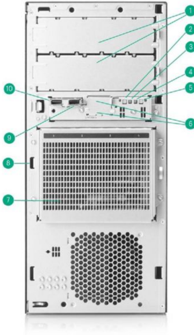
Front View 4LFF Gen11
